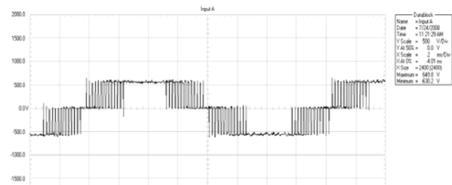
Fig. 1. PWM voltage measured at VFD output terminals [3,4]
