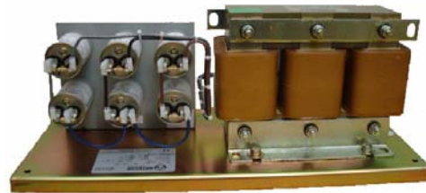
Fig. 5. Sine Wave dv/dt Filter: photo compliments of Artech.
