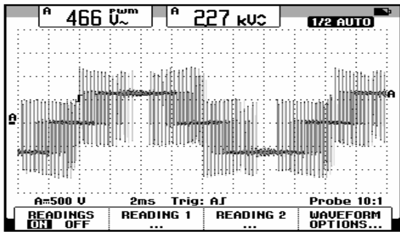
Fig. 2. Motor terminal voltage measurement
